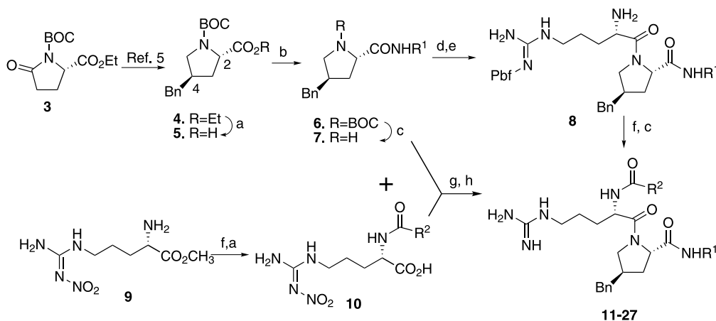
Scheme 1. Synthesis of trans proline analogs. Reagents and conditions: (a) LiOH, CH 3 OH/H 2 O, 18 h, 92%; (b) R 1 NH 2 , EDCI, HOBT, NMM, DMF, 4 h, 54–79%; (c) TFA/CH 2 Cl 2 , 3 h, ~100%; (d) Pbf-(Fmoc)-Arg-OH, EDCI, HOBT, NMM, DMF, 4 h, ~90%; (e) piperidine, DMF, 0.5 h, ~91%; (f) R 2 CO 2 H, EDCI, NMM, HOBT, DMF, 3 h, 61–81%; (g) EDCI, HOBT, NMM, DMF, 5 h, 54–62%; (h) H 2 , Pd/BaSO 4 , HOAc, CH 3 OH, 10 h, 30–50%.
