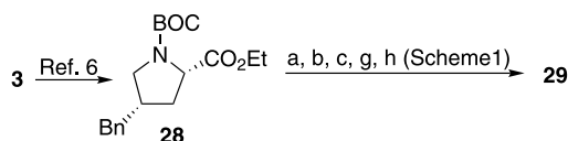
Scheme 2. Synthesis of cis proline analogs.
