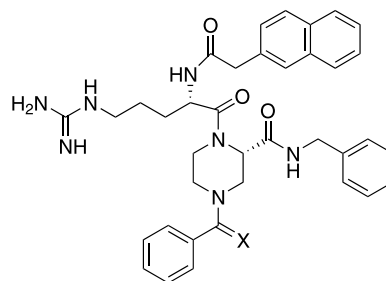
1. X=H 2 , K i =376 nM at MC4R; 2. X=O, K i =649 nM at MC4R.
