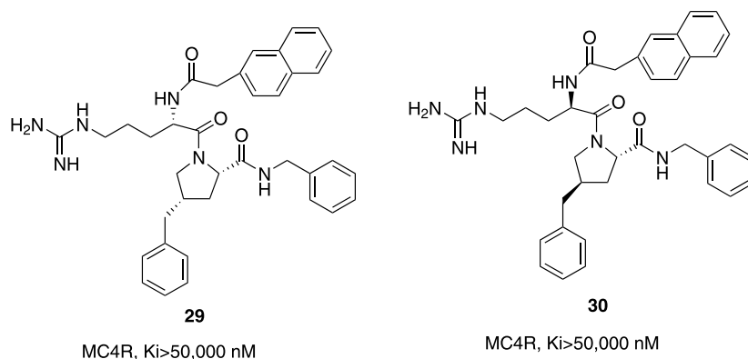
Figure 3. Stereochemical effect on affinity.
