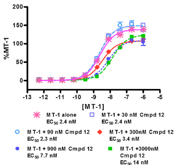
Figure 2. MT-1 dose response curves \pm compound 12 : luciferase response in MC4cre Cells.
